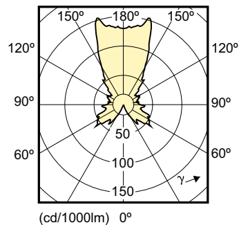
SDLD_LEDLSR_0023-Light distribution diagram
